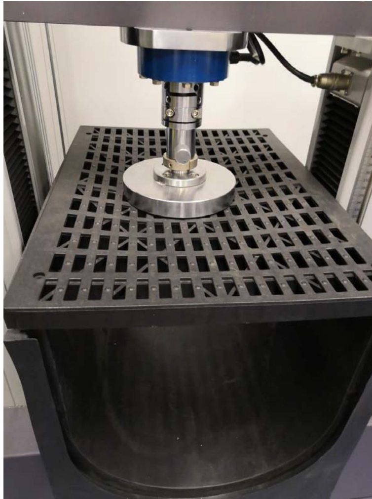
Fig.2 Picture of sample during load-bearing test
